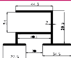
I-SKP-24 Aluminio Aluminium
