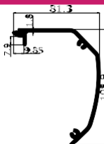
İ-SKP-28 Aluminio Aluminium
